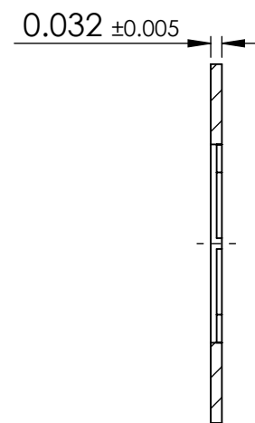
SECTION Y-Y
